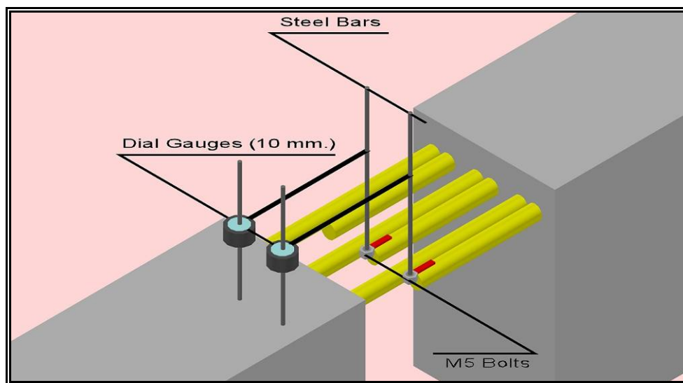
Figure 3.13 Detailed view for slip measurement.
