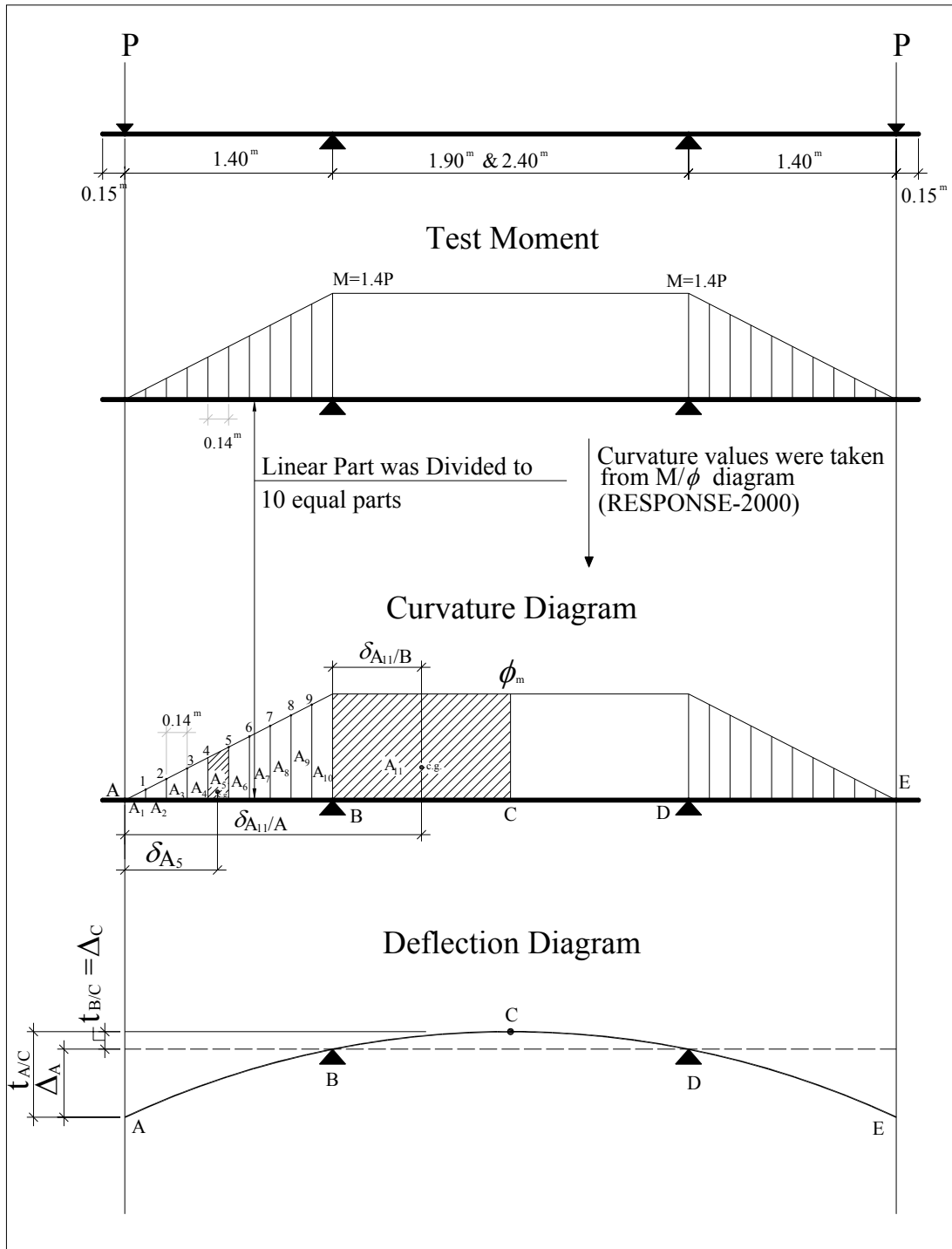
Figure 5.1 Procedure for calculating Load – Deflection Curves.
