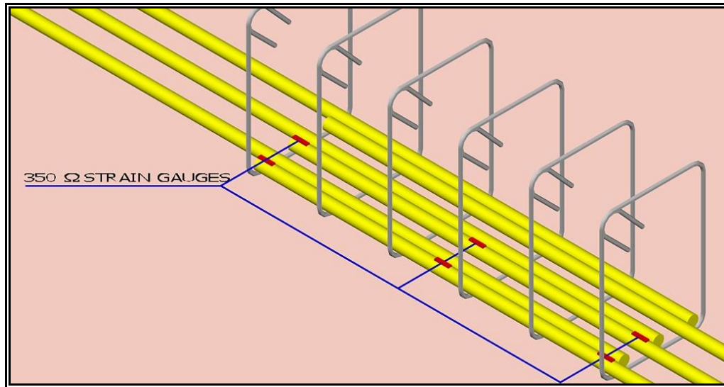
Figure 3.15 Detailed view for location of 350 \Omega strain gauges.
