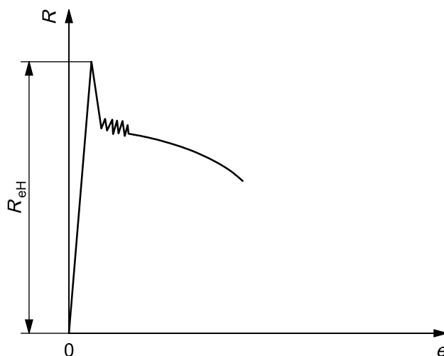
c) Special case of stress-percentage extension behaviour a
